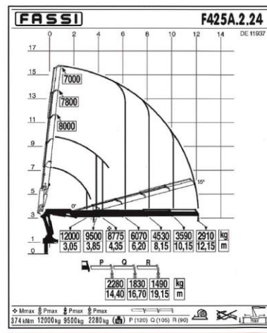
FASSI F425A.2.24 e-dynamic - Load Diagram LOAD DIAGRAM WITH LIFTING MOMENT LIMITING DEVICE
